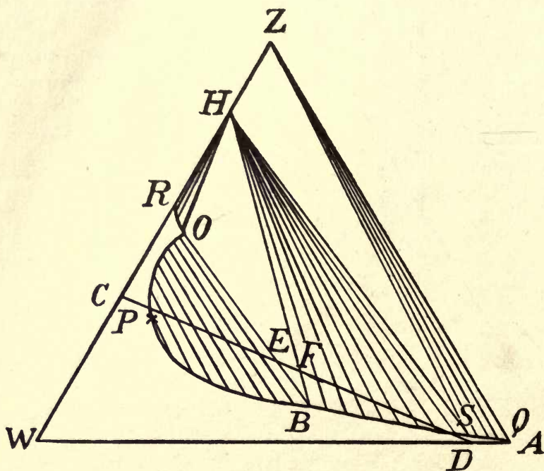
Figure 8. B. de Bruyn's Diagram for the System: Potassium Carbonate, Methyl Alcohol, Water.
